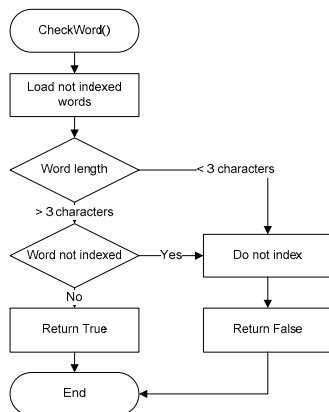
Figure 2. Algorithm model checks the words
