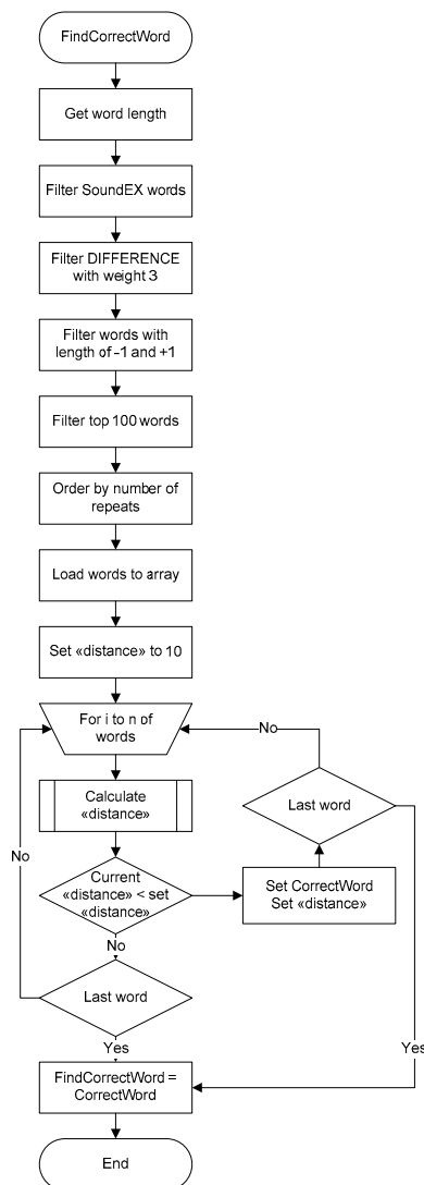
Figure 4. Model of correction algorithm of the searched term
