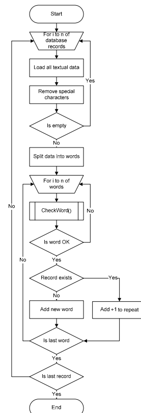
Figure 1. Indexing algorithm model
