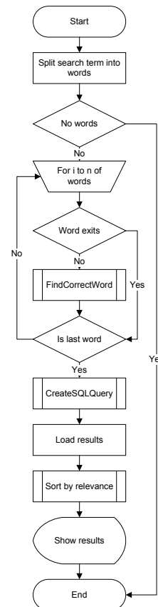
Figure 3. Search algorithm model
